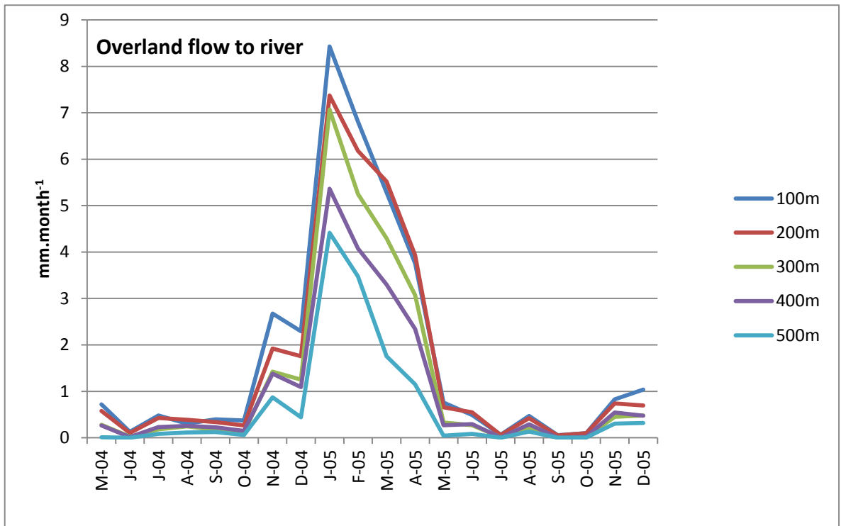
Figure 7. Simulated overland flow winter/spring period
