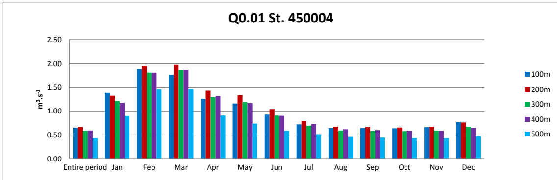
Figure 11. Monthly values for 1 pct discharge (Q0.01, median) calculated from daily data for period 2002-2007 for discharge station 450004 (302 km 2 ). First columns are averaged for entire period.
