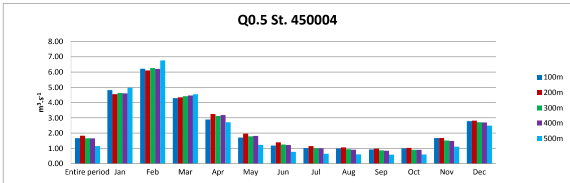
Figure 13. Monthly values for 50 pct discharge (Q0.50) calculated from daily data for period 2002-2007 for discharge station 450004. First columns are averaged for entire period.
