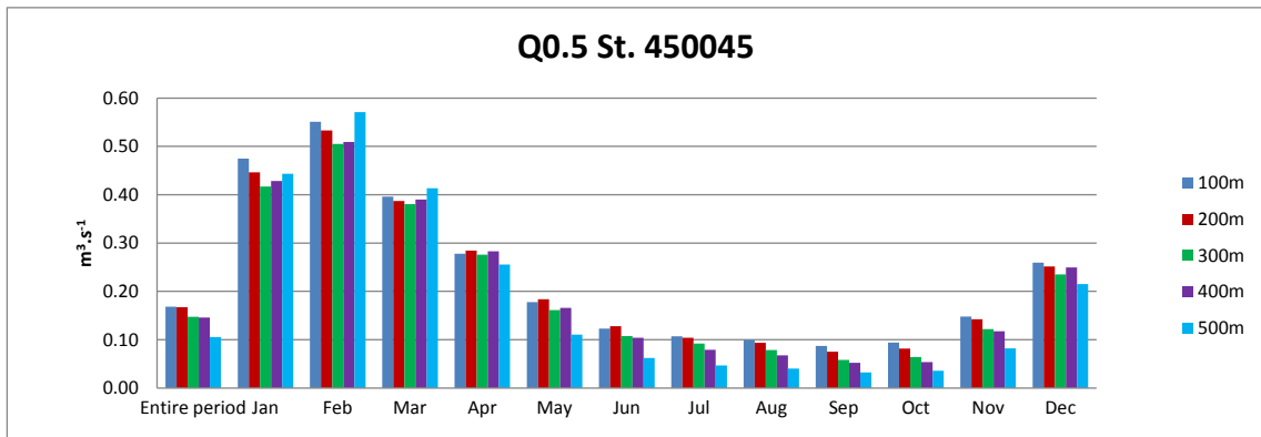
Figure 12. Monthly values for 50 pct discharge (Q0.50) calculated from daily data for period 2002-2007 for discharge station 450045. First columns are averaged for entire period.
