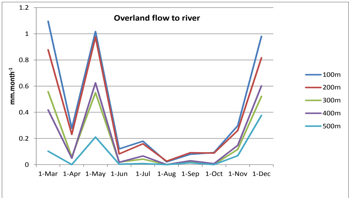
Figure 8. Simulated overland flow summer 2003. Lower grid size sustains higher overland flow.
