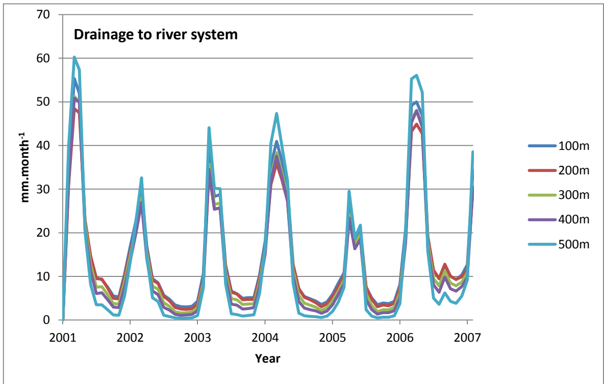
Figure 5. Seasonal variation in drainage to the river system for the sub catchment.
