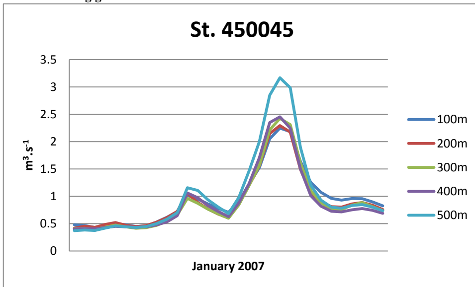
Figure 18. Discharge for January 2007 at station 450045 for grid sizes 100-500. Increasing discharge with increasing grid size.
