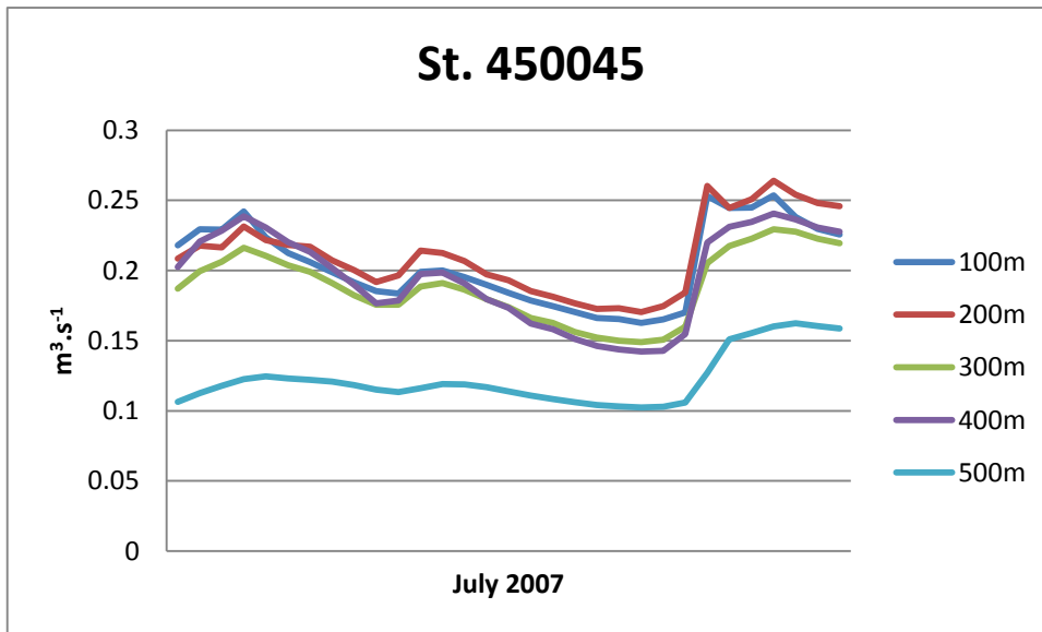
Figure 19. Discharge for July 2007 at station 450045 for grid sizes 100-500. Increasing discharge with decreasing grid size.
