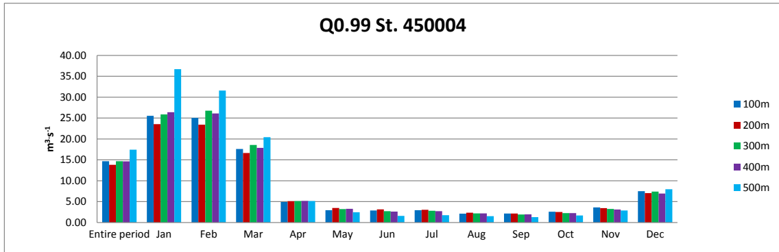
Figure 15. Monthly values for 99 pct discharge (Q0.99) calculated from daily data for period 2002-2007 for discharge station 450004. First columns are averaged for entire period.
