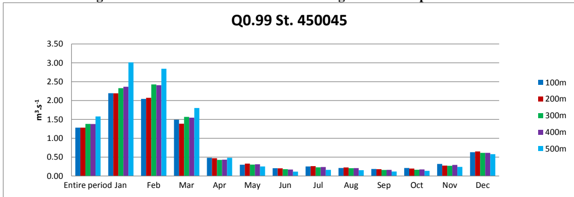
Figure 14. Monthly values for 99 pct discharge (Q0.99) calculated from daily data for period 2002-2007 for discharge station 450045. First columns are averaged for entire period.
