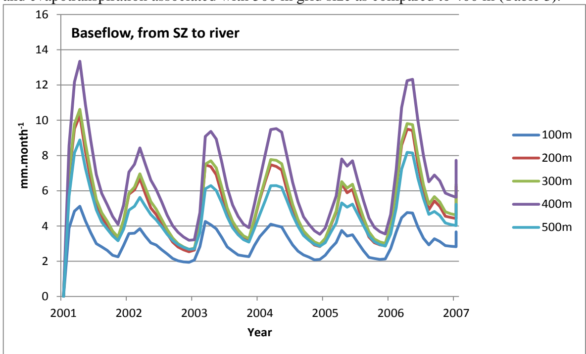
Figure 9. Simulated base flow from SZ to river for sub catchment.
