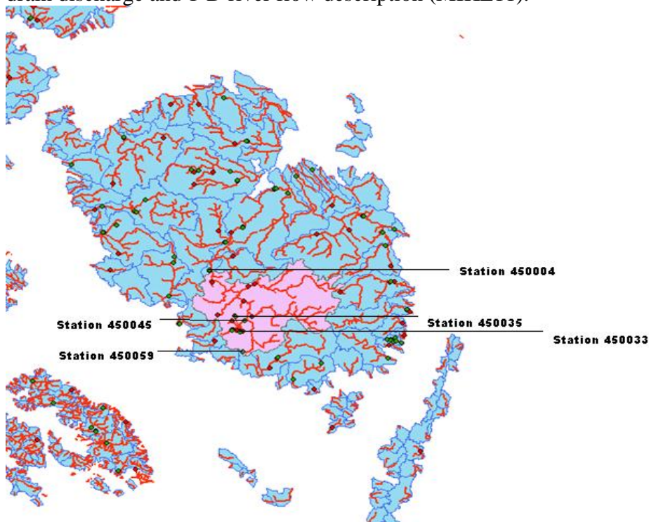
Figure 1. Sub-catchment is upstream of discharge station 450004 and included as model domain in MIKE SHE. Discharge stations 450004 (draining 302 km 2 ), 450045 (draining 30.2 km 2 , 450033 (3.51 km 2 ), 450035 (2.56 km 2 ) and 450059 (0.38 km 2 ) are also indicated
