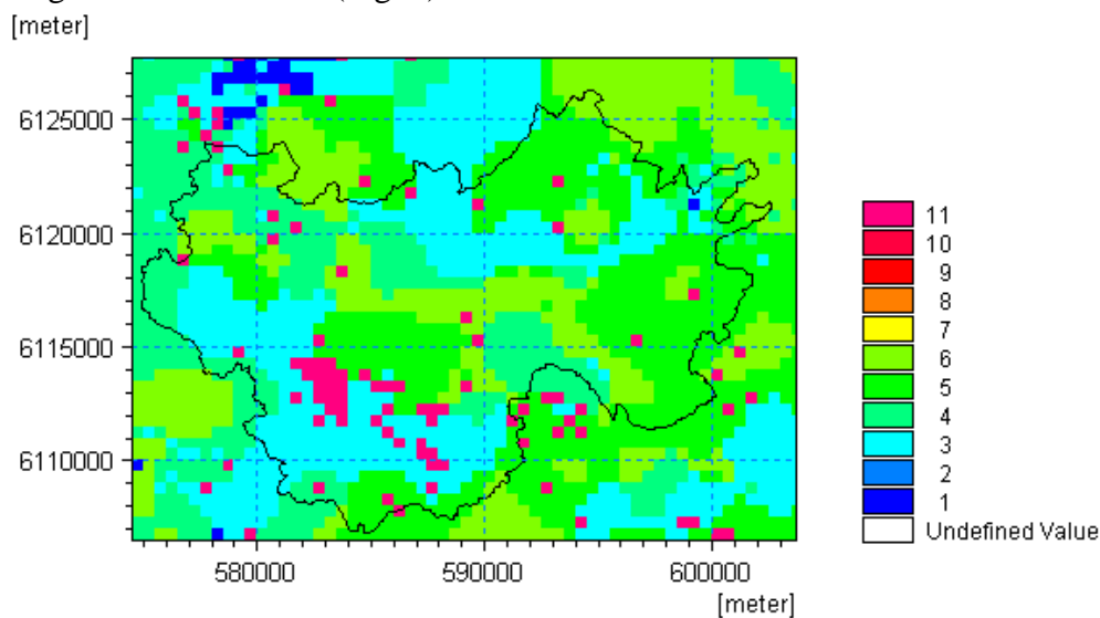
Figure 4. Spatial distribution of soil classification and associated hydraulic properties in the unsaturated zone. Refer to Table 1 for grid codes and assigned soil hydraulic properties. Some codes in the legend (2,7,8,9,10) do not occur in the sub-catchment
