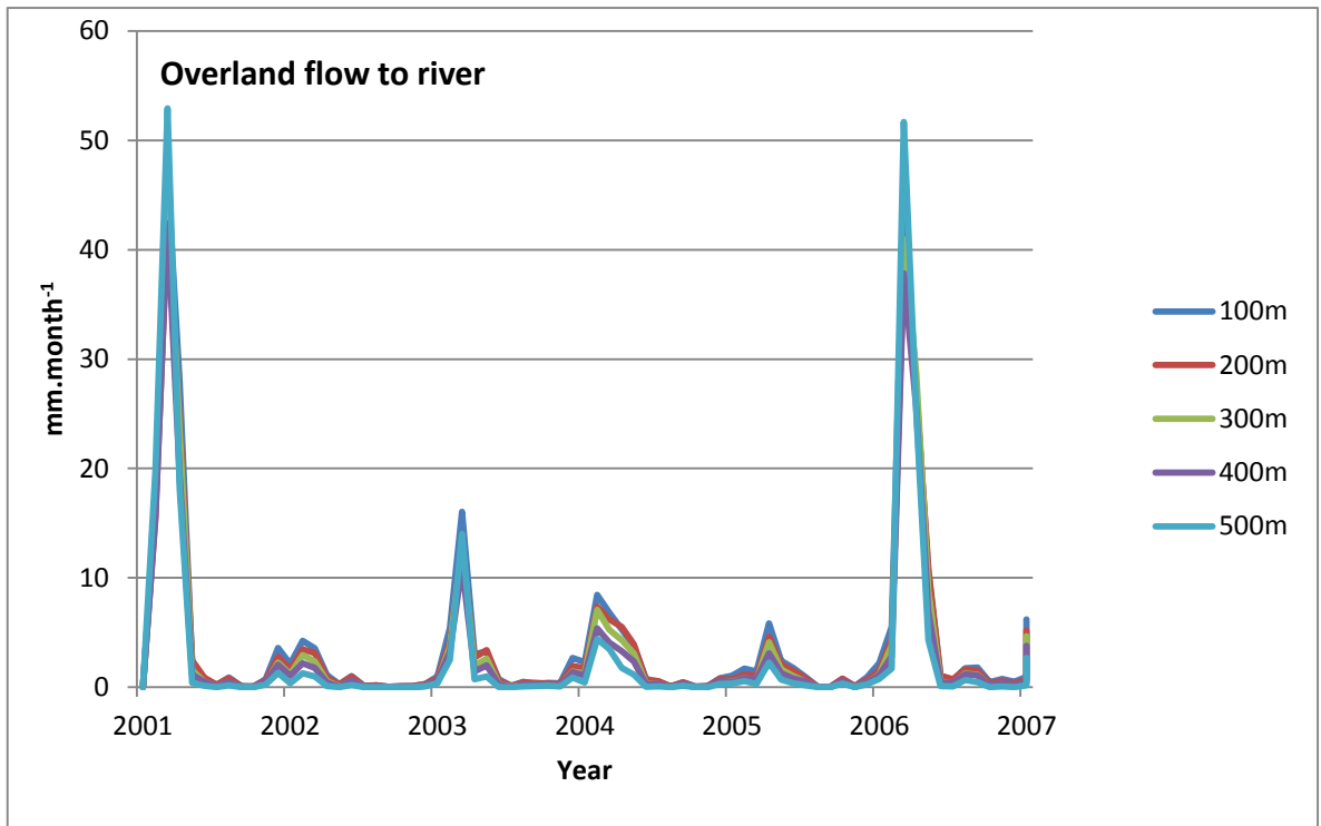
Figure 6. Simulated overland flow to river for the sub catchment
