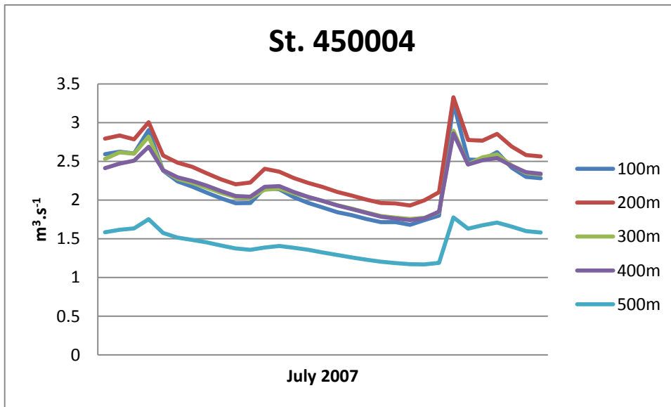
Figure 17. Discharge for July 2007 at station 450004 for grid sizes 100-500. Increasing discharge with decreasing grid size.
