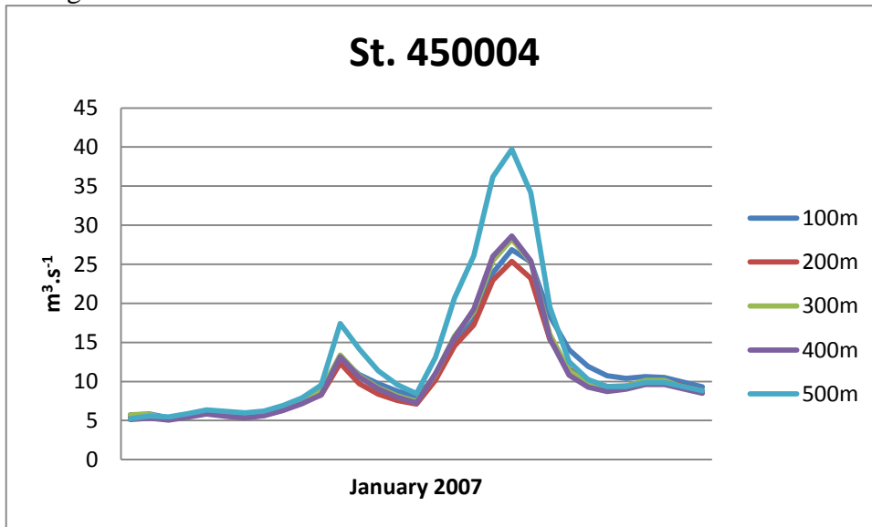
Figure 16. Discharge for January 2007 at station 450004 for grid sizes 100-500. Increasing discharge with increasing grid size.
