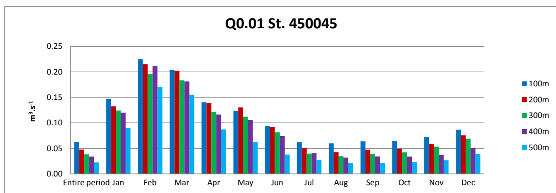
Figure 10. Monthly values for 1 pct discharge (Q0.01) calculated from daily data for period 2002-2007 for discharge station 450045 (30.2 km 2 ). First columns are averaged for entire period.
